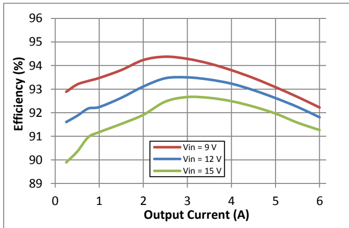
Fig. 3 Efficiency vs Output Current
