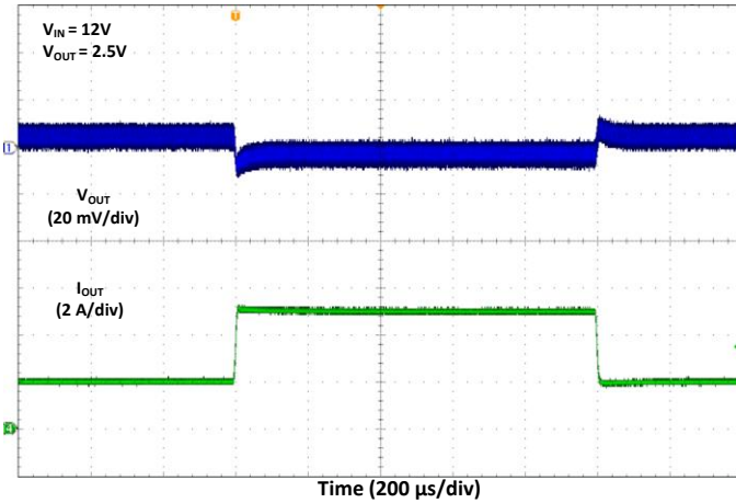
Fig. 29 SPM1004-2V5, V_{IN} = 12V , V_{OUT} = 2.5V
