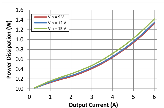
Fig. 12 Power Dissipation vs Output Current
