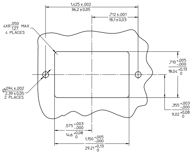
RECOMMENDED MOUNTING PATTERN
