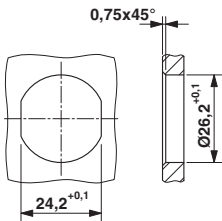
Drilling diagram
