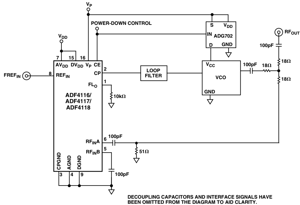
Figure 8. Local Oscillator Shutdown Circuit
