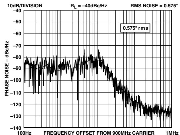
TPC 5. ADF4118 Integrated Phase Noise (900 MHz, 200 kHz, 20 kHz, Typical Lock Time: 400 \mu s)
