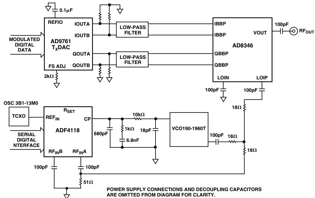
Figure 9. Direct Conversion Transmitter Solution
