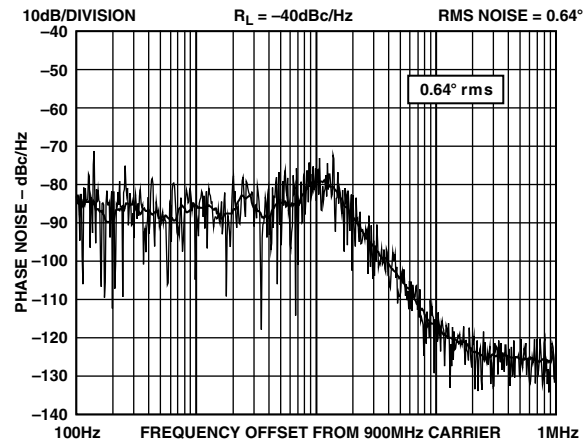
TPC 4. ADF4118 Integrated Phase Noise (900 MHz, 200 kHz, 35 kHz, Typical Lock Time: 200 \mu s)
