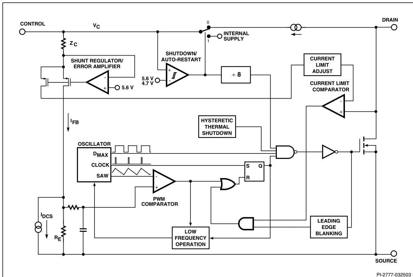
Figure 2. Block Diagram.
