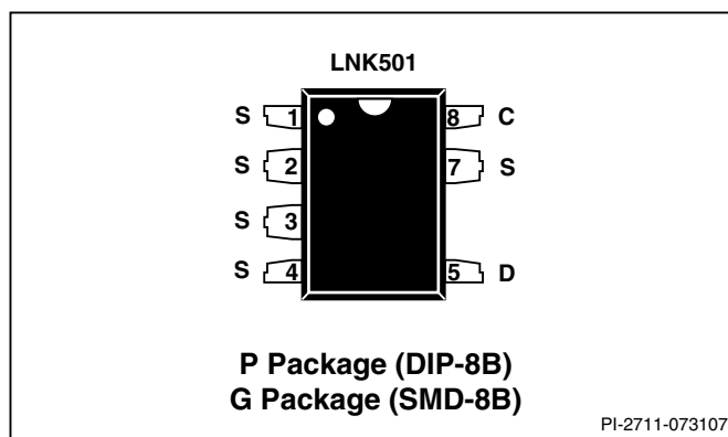
Figure 3. Pin Configuration.
