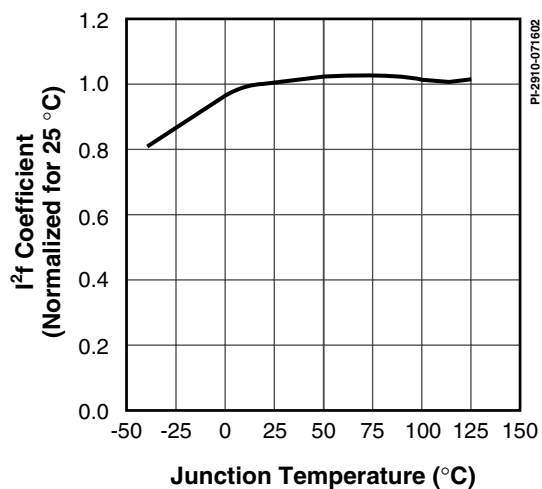
Figure 20. I^2t Coefficient vs. Temperature.
