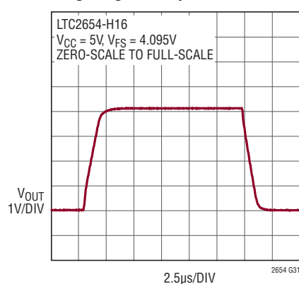
Large-Signal Response
