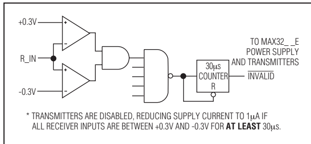
Figure 3a. MAX32_E Entering 1\mu\text{A} Supply Mode via AutoShutdown
