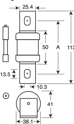
Figs. 4 &amp; 5 "A" Dimensions
