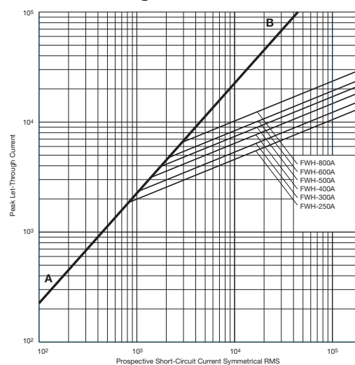
Peak Let-Through Curve
