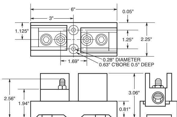
Figure 5. 300V, 600V 101 to 200A
