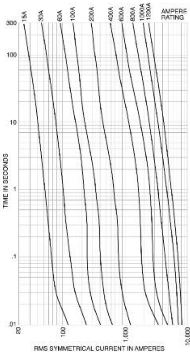
Average Time-Current Curve Cat. No. TJN (Amp)
