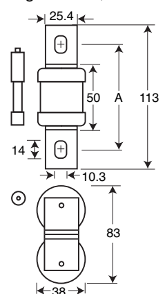
Figs. 4 &amp; 5 "A" Dimensions
