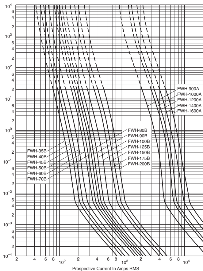
Time-Current Curve
