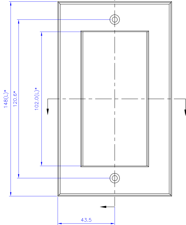
FRONT ELEVATION
