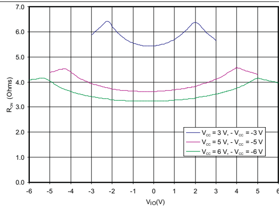
Figure 1. R_{ON} vs V_{IO}
