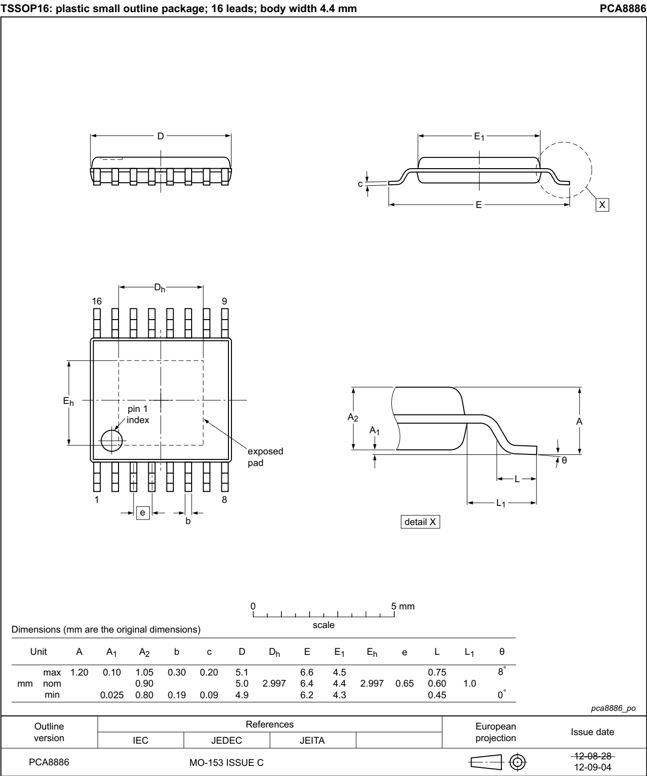
Fig 16. Package outline of PCA8886TS (TSSOP16)
