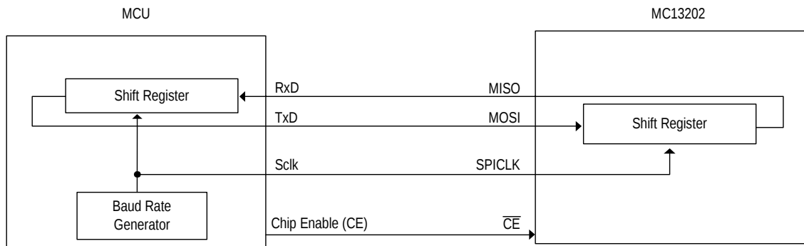
Figure 7. SPI Interface
