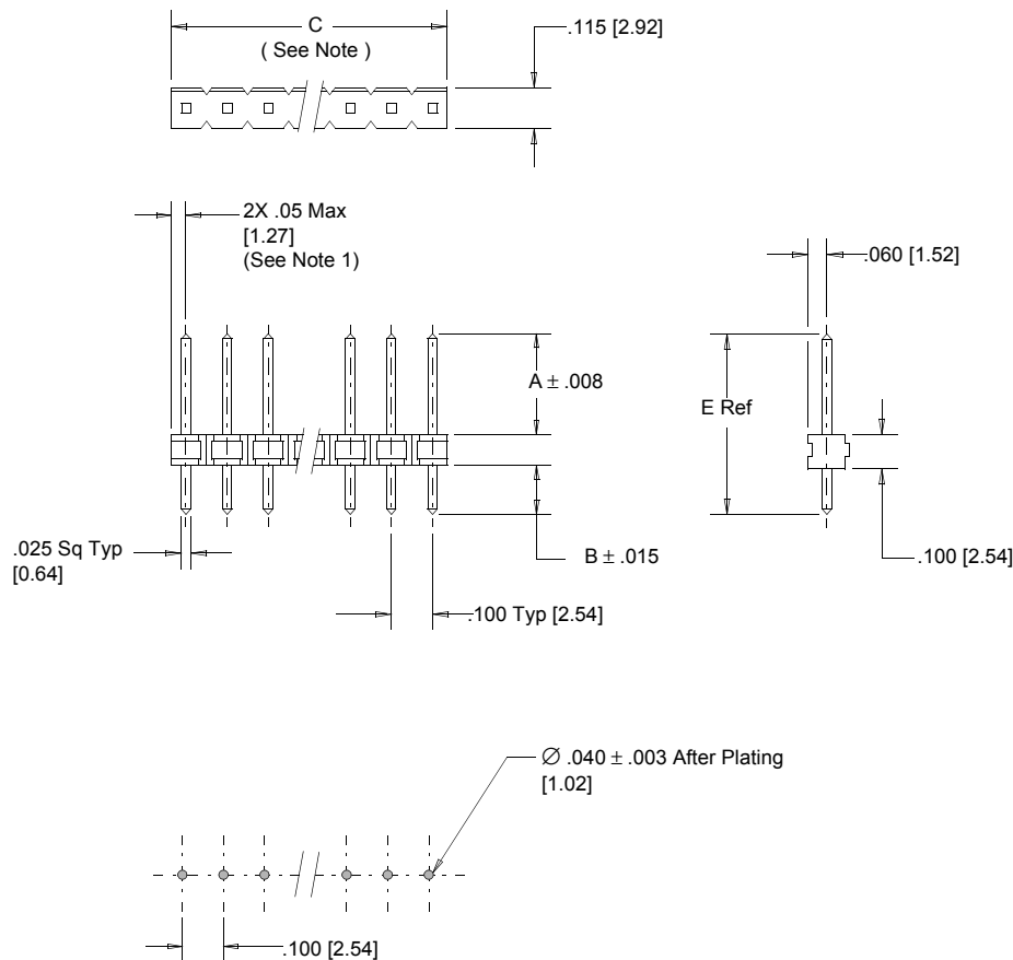
Recommended Hole Pattern
