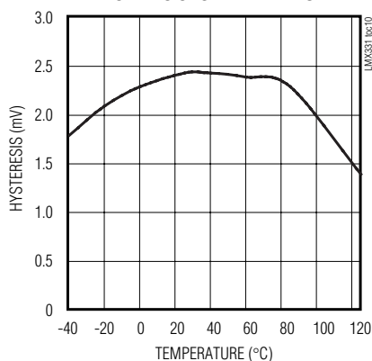
LMX331H/LMX339H/LMX339H HYSTERESIS vs. TEMPERATURE
