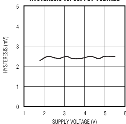
LMX331H/LMX339H/LMX339H HYSTERESIS vs. SUPPLY VOLTAGE
