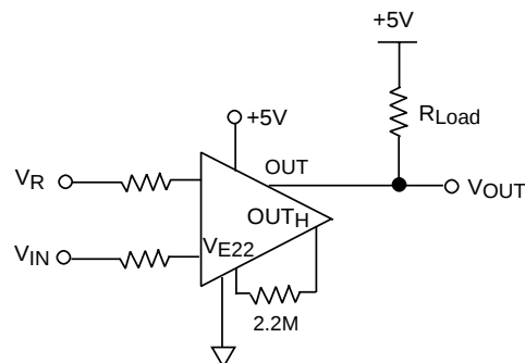
VOLTAGE COMPARATOR WITH OUTPUT FEEDBACK TO PROVIDE HYSTERSIS
