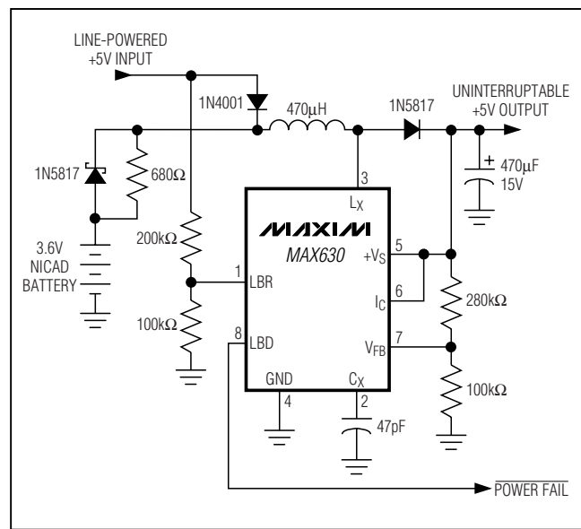
Figure 6. Uninterruptable +5V Supply
