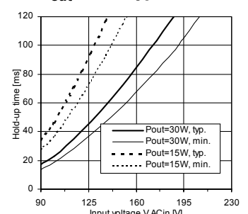
Hold-up time with ACin (at V_{out} = 10\text{V} , typ. + min.)
