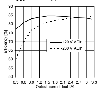
Efficiency (@ V_{out} = 10\text{V} , typ.)
