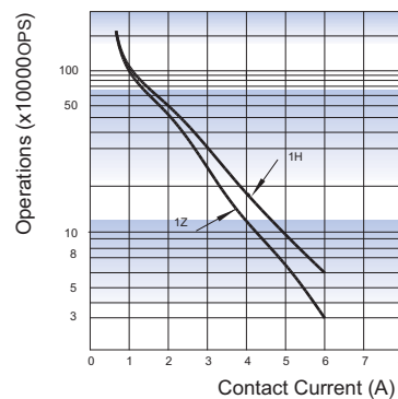
ENDURANCE CURVE
