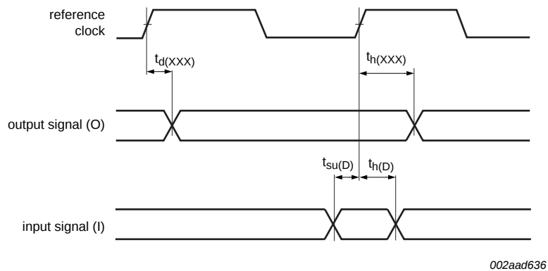
Fig 18. Signal timing
