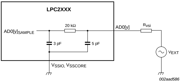
Fig 20. Suggested ADC interface - LPC2468 AD0[y] pin
