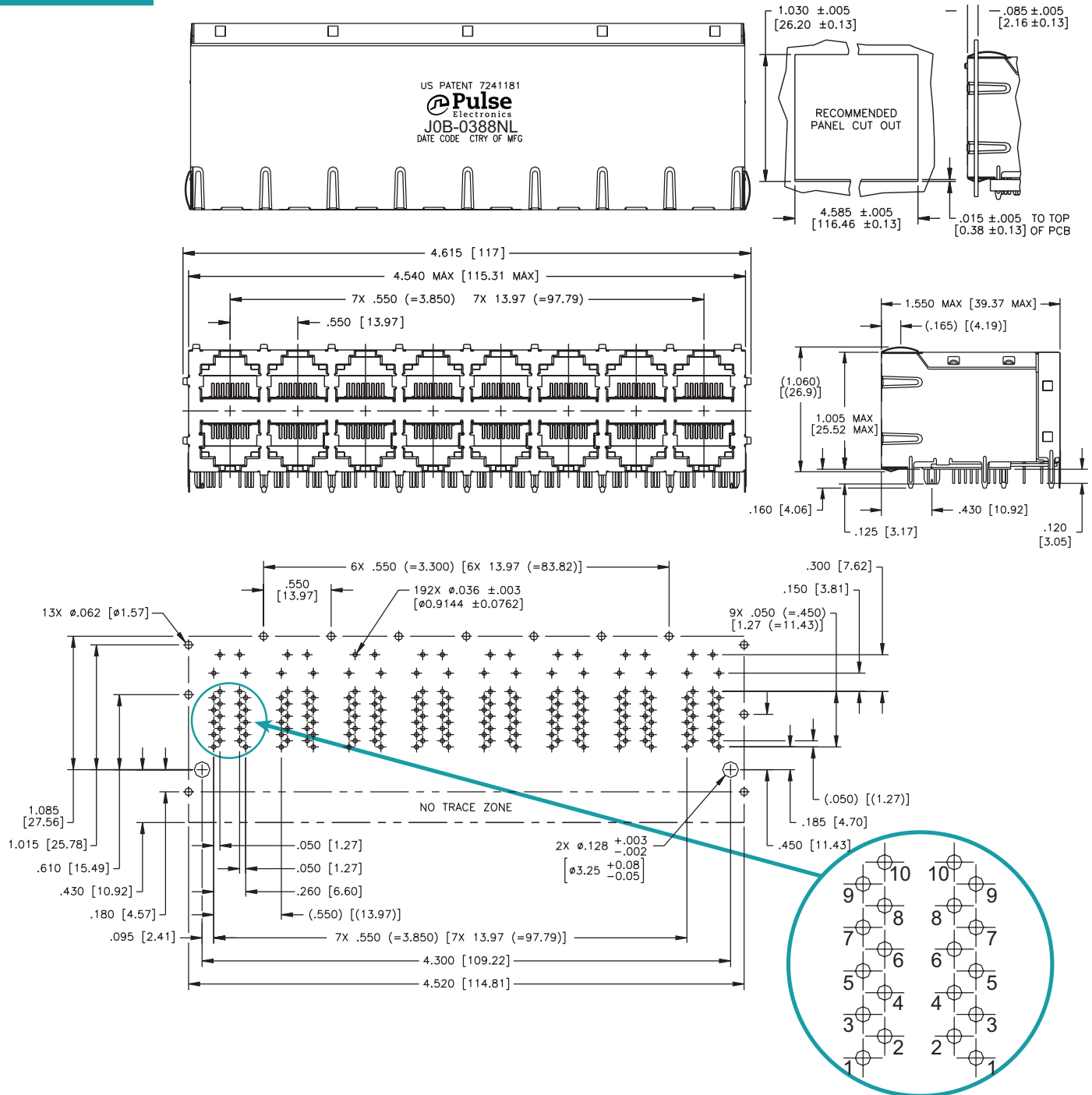
Pin-out Assignment
