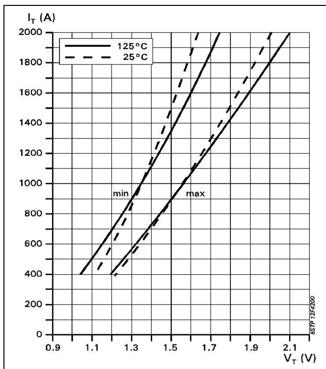
Fig. 2 On-state characteristics.
