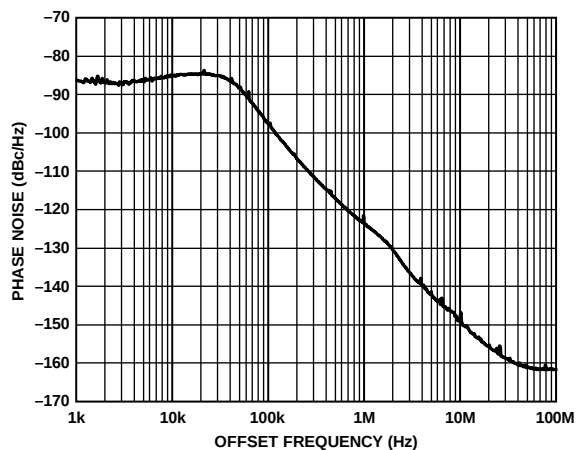
Figure 16. Transmit Synthesizer Phase Noise
