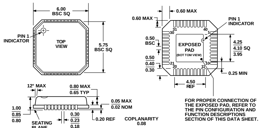
Figure 47. 40-Lead Lead Frame Chip Scale Package [LFCSP_VQ] 6 mm × 6 mm Body, Very Thin Quad (CP-40-1)
