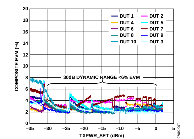
Figure 7. Transmit EVM vs. TXPWR_SET (dBm), Measured Across 10 DUTs, Four Calibration Points Applied
