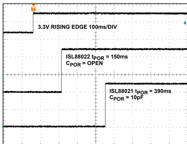
FIGURE 6. ISL88021_22EVAL1 t_{POR} COMPARISON
