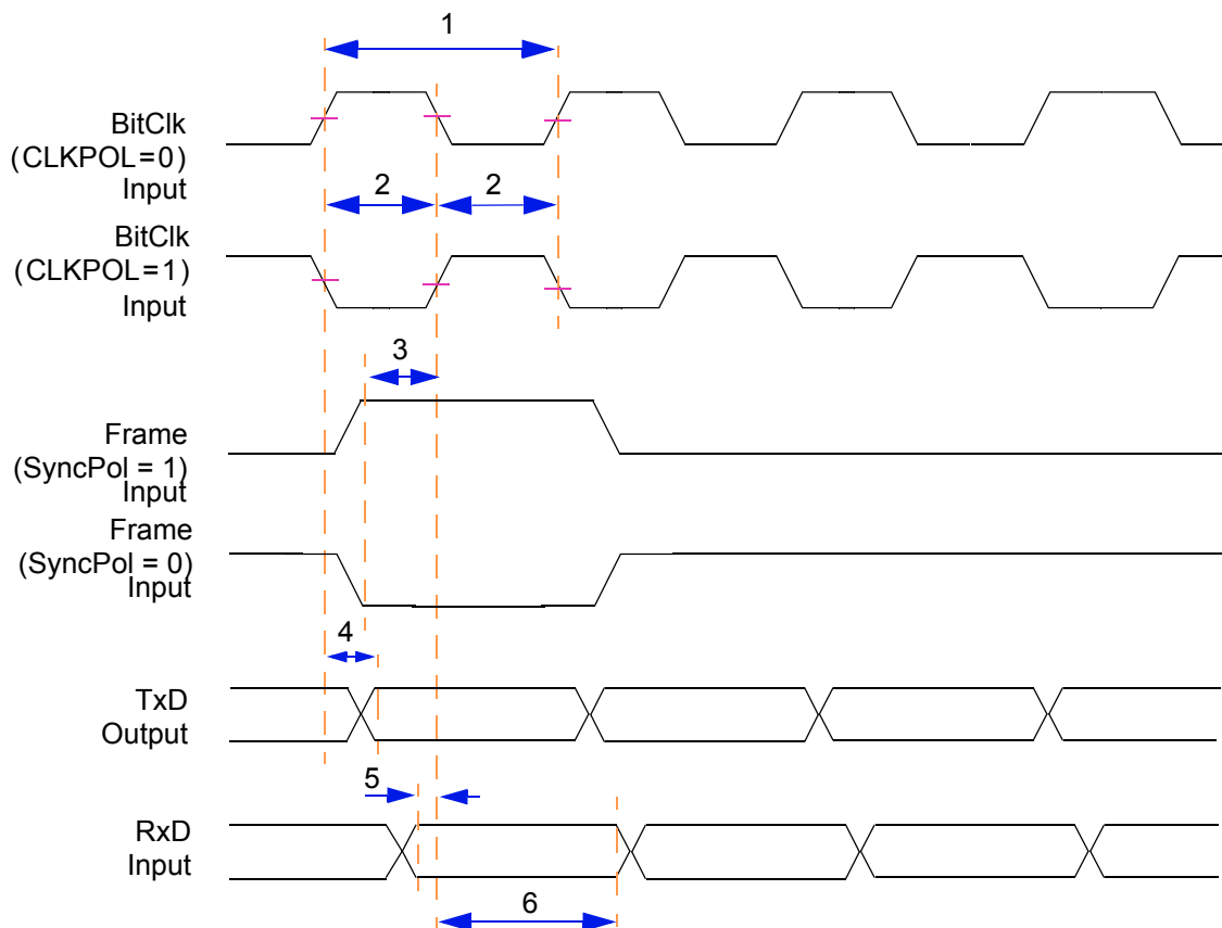
Figure 39. Timing Diagram — 8,16, 24, and 32-bit CODEC / I²S Slave Mode
