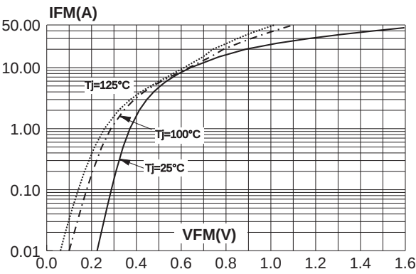
Fig. 7-2: Forward voltage drop versus forward current (typical values) (1N5822).
