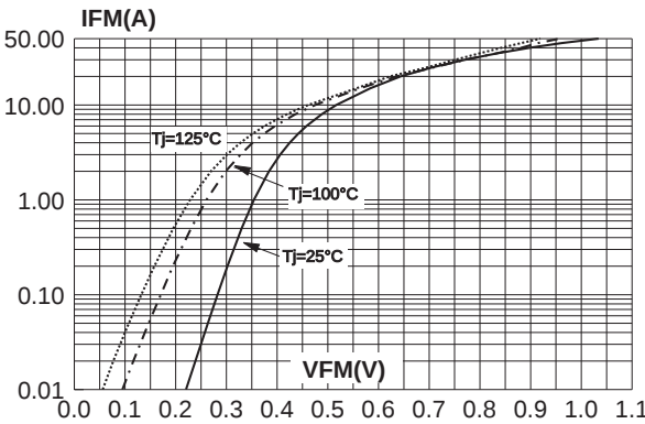
Fig. 7-1: Forward voltage drop versus forward current (typical values) (1N5820/1N5821).
