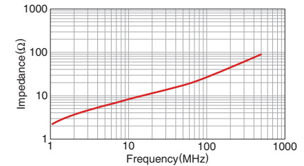
HF70SH18.5X0.7X6
