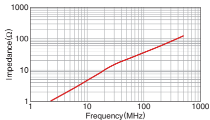
HF40SH18.5X0.7X8-G
