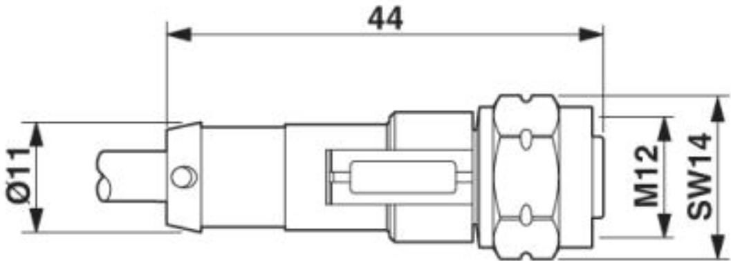
M12 x 1 socket, straight
