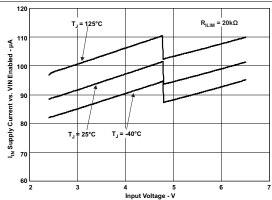
Figure 8. I_{IN} – Supply Current, Output Enabled – \mu A
