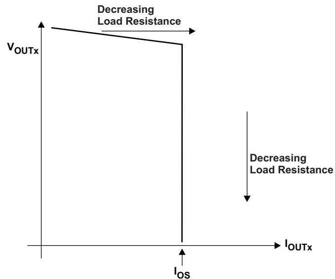
Figure 14. Output Voltage vs Current-Limit Threshold
