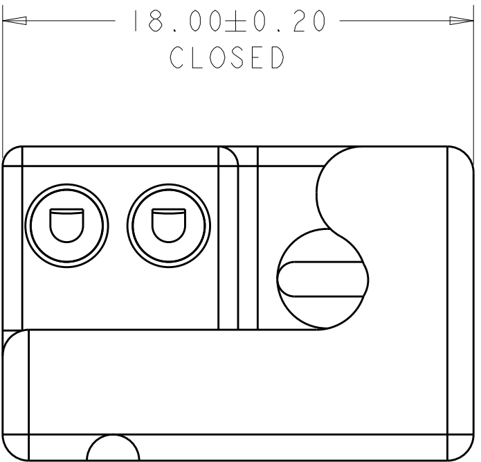
TERMINATED DETAIL
