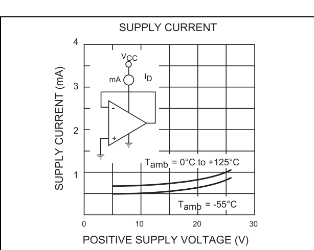
Figure 12. Supply current
