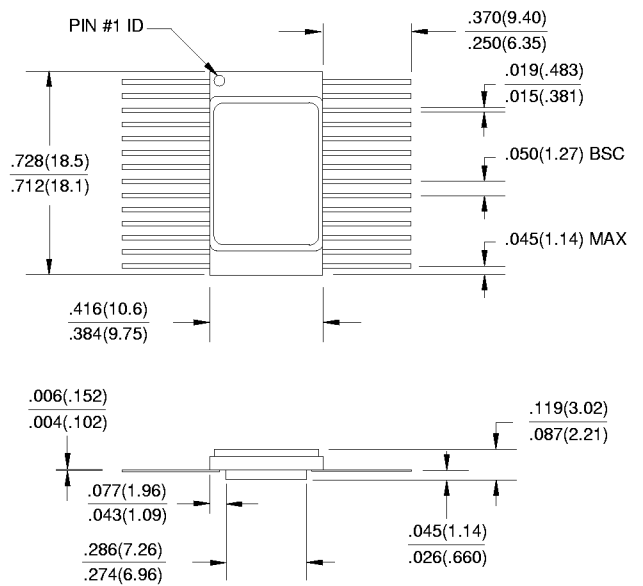
28F , 28-Lead, Non-Windowed, Ceramic Bottom- Brazen Flat Package (Flatpack) Dimensions in Inches and (Millimeters) MIL-STD-1835 F-12 CONFIG B
