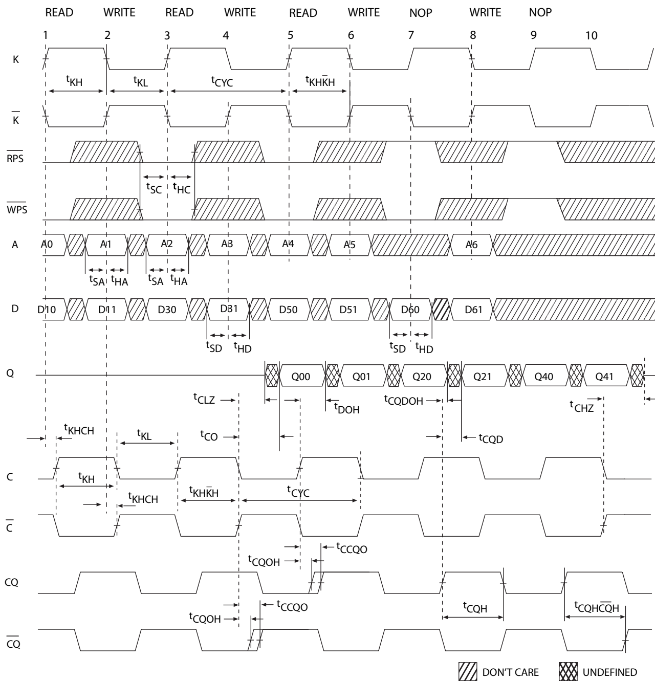
Figure 5. Read/Write/Deselect Sequence [26, 27, 28]
