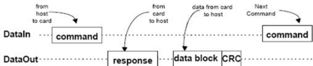
Figure 7-3: Single Block Read operation
