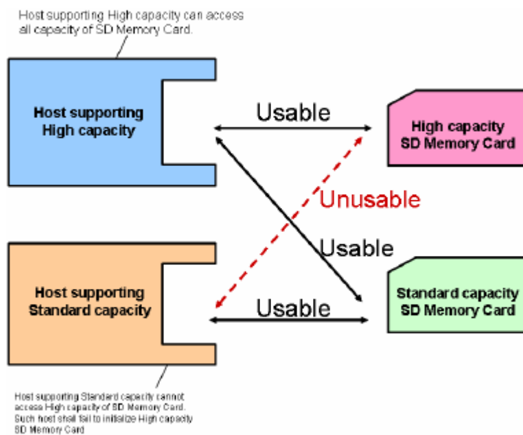
Figure 4-5: Hosts-Cards Usability
