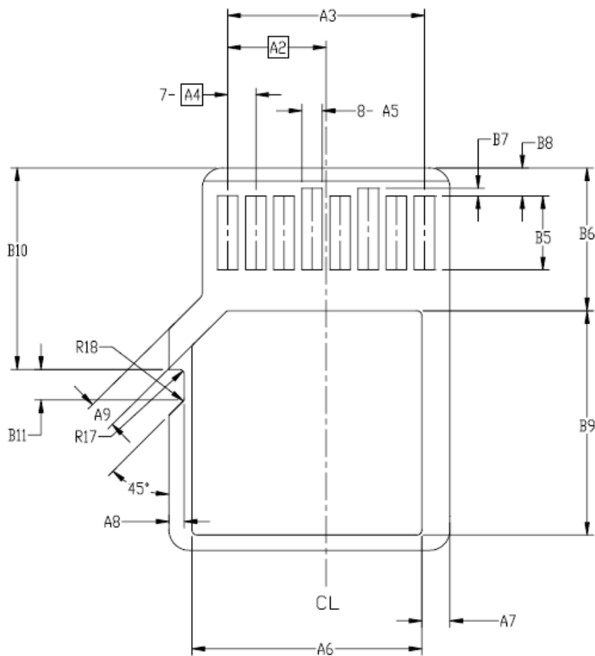
Figure 2-11: Dimensions of microSD (Bottom View)
