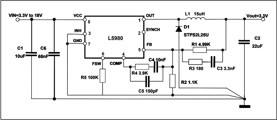
Figure 18. Demonstration board application circuit
