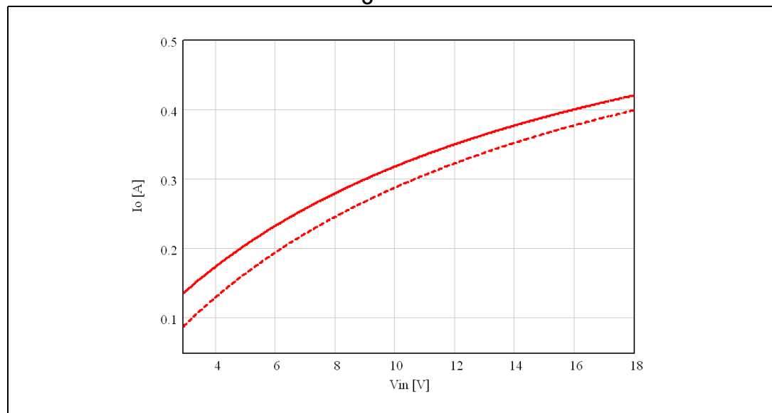
Figure 32. Maximum output current according to max DC switch current (0.7 A): V_O = 12\text{ V}
