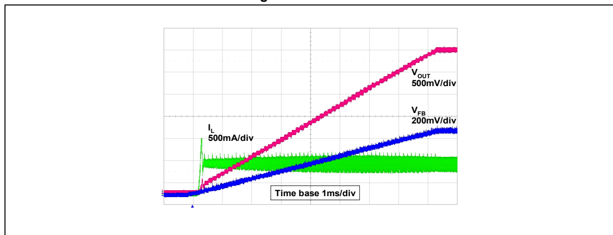
Figure 30. Soft-start
