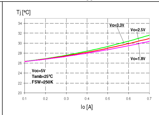
Figure 23. Junction temperature vs. output current - V_{CC} = 5\text{ V}
