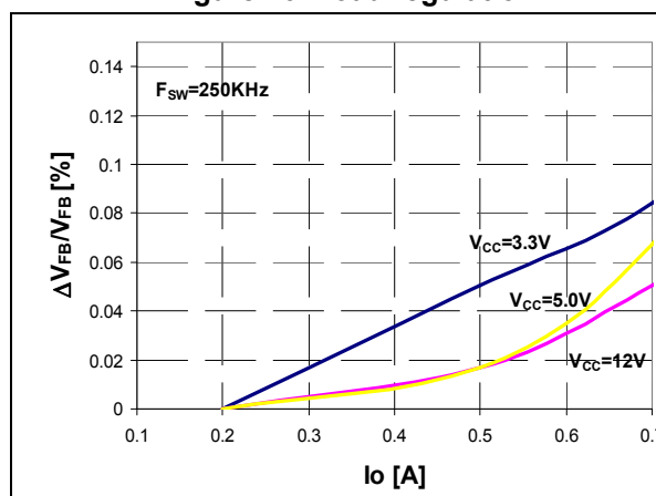
Figure 26. Load regulation
