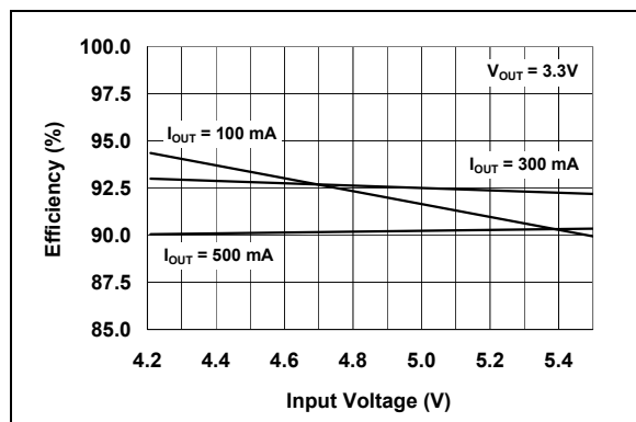
FIGURE 2-7: Efficiency vs. Input Voltage ( V_{OUT} = 3.3\text{V} ).
