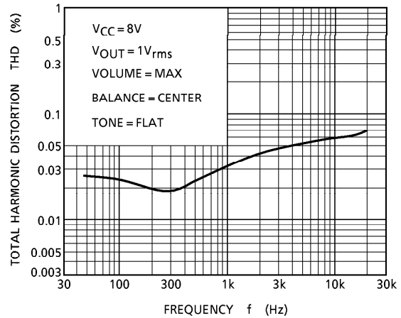
THD - f
