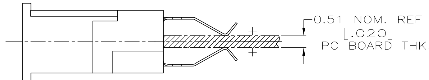
PC BOARD LOCATION (REF) SCALE: 10:1
