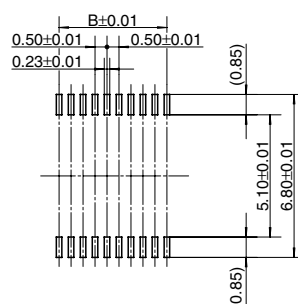
Recommended metal mask pattern
