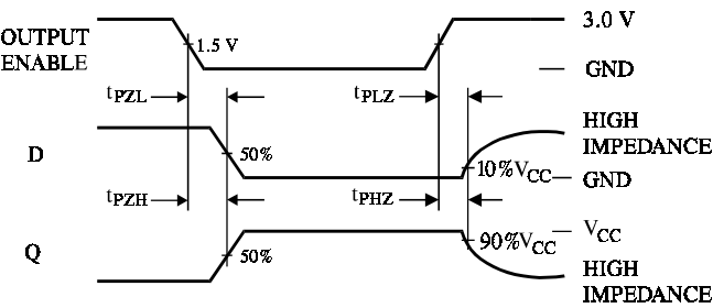
Figure 2. Switching Waveforms
