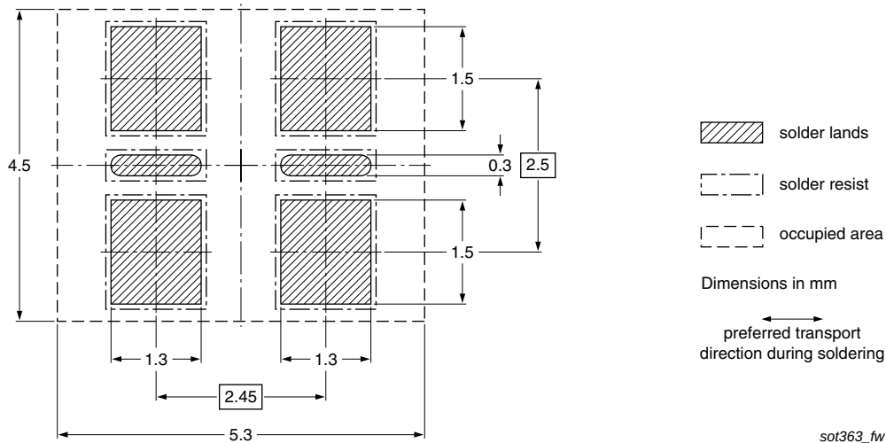
Fig 27. Wave soldering footprint SOT363 (SC-88)
