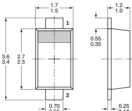
Fig 6. Package outline SOD523 (SC-79)
