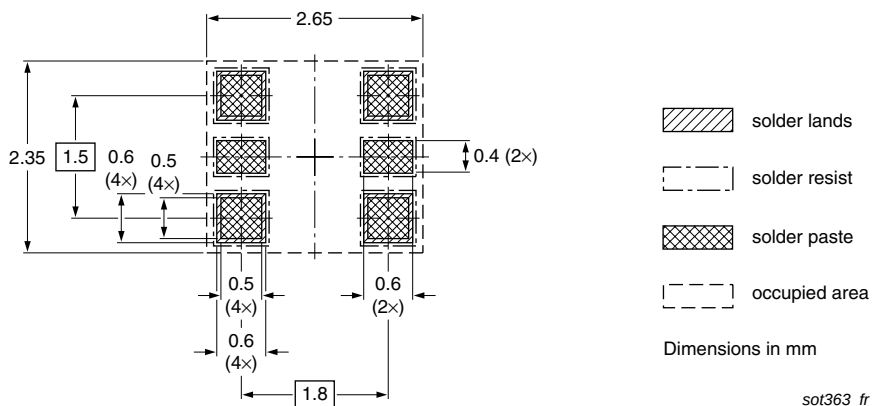
Fig 26. Reflow soldering footprint SOT363 (SC-88)
