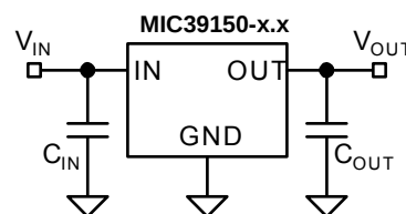
Figure 1. Capacitor Requirements
