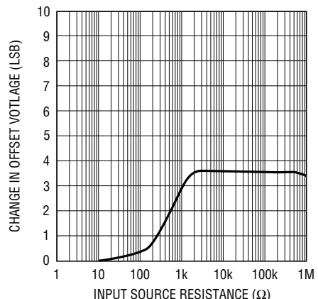
Input Offset Voltage Shift vs Source Resistance
