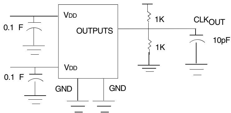
TEST CIRCUIT 1
