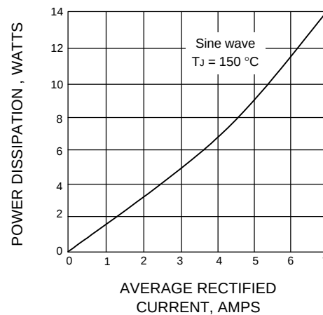
FIG.4 - POWER DISSIPATION
