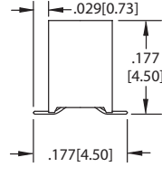
DUAL ROW, SMT Without Guide Posts (NFSS)
