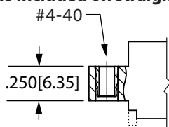
THREADED INSERT (I)
