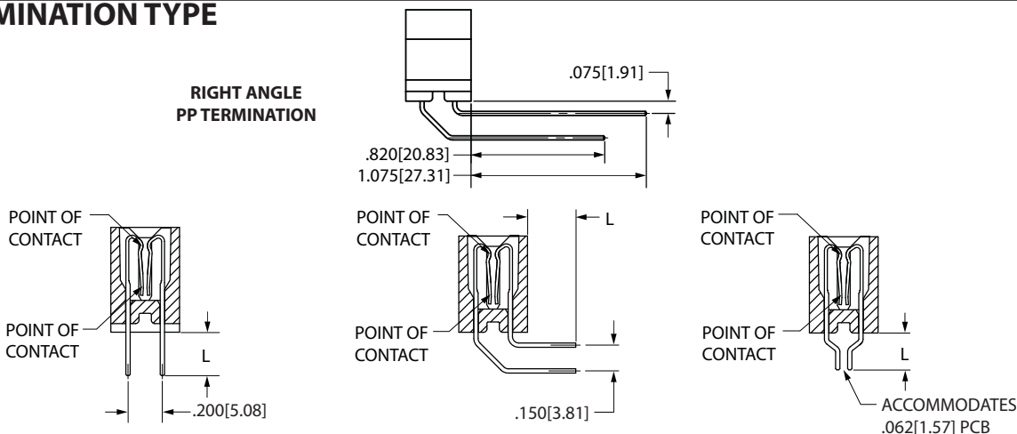
DIP SOLDER/WIRE WRAP (PD, PF, PS, PM)
