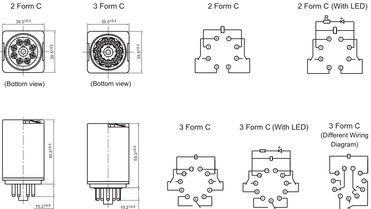
Wiring Diagram (Bottom view)
