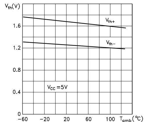
Figure 8: Receiver threshold vs temperature
