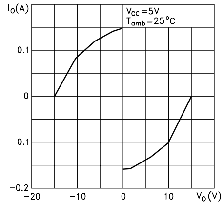
Figure 6: Driver output capability current vs output voltage
