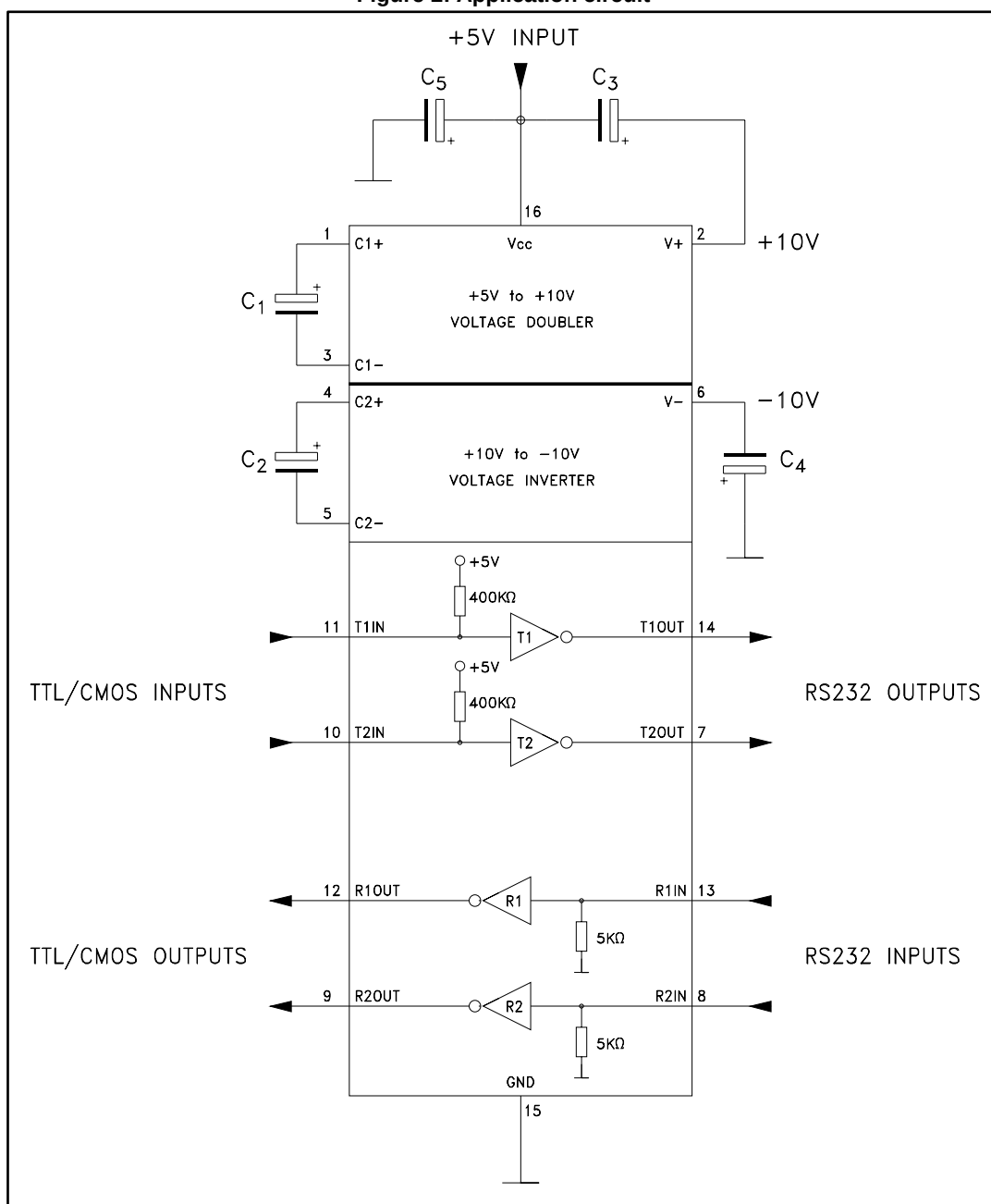
Figure 2: Application circuit
