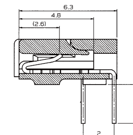
SECT. X-X
