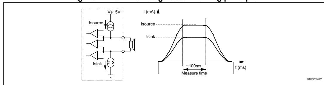
Figure 22. Turn - on diagnostic: working principle
