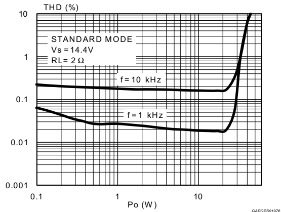
Figure 9. Distortion vs. output power (2 \Omega , STD)
