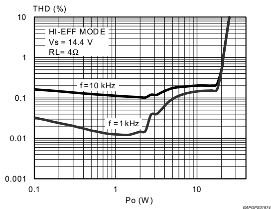
Figure 8. Distortion vs. output power (4 \Omega , HI-EFF)
