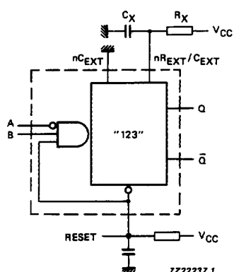
Fig.11 Power-up output pulse elimination circuit.
